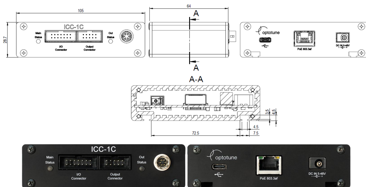
Figure 2: Mechanical dimensions, front and back panel overview of the ICC-1C
