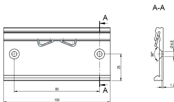
Figure 3: DIN rail adapter
